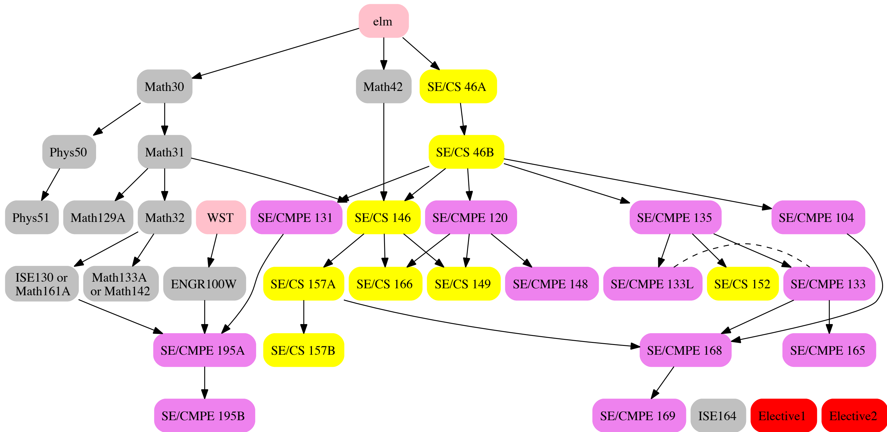
Prerequisite relationships for the BS SE degree, 2006-2008 catalog.
